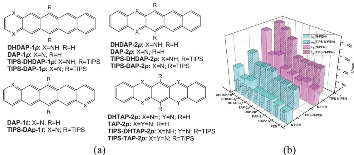
Fig. 4 (a) Molecular structures of the systems investigated, (b) the reorganization energies evaluated from the adiabatic potential-energy surface. Reprinted from ref. 60 with permission from The Royal Society of Chemistry.
