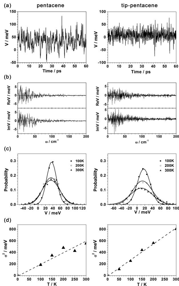
Fig. 7 (a) Thermal fluctuation of the transfer integral (dimer A) for pentacene (left) and tips-pentacene (right) at 300 K; (b) Fourier transformation of thermal fluctuation amplitude (ReV and ImV) at 300 K; (c) probability distribution of the transfer integral V of dimer A. The solid line represents a Gaussian fit. (d) Square of the standard deviation of transfer integral as a function of temperature. (left) Reproduced from ref. 48 with permission from the Royal Society of Chemistry. (right) Reprinted with permission from ref. 56. Copyright © 2012 Wiley-VCH Verlag GmbH & Co. KGaA, Weinheim.
